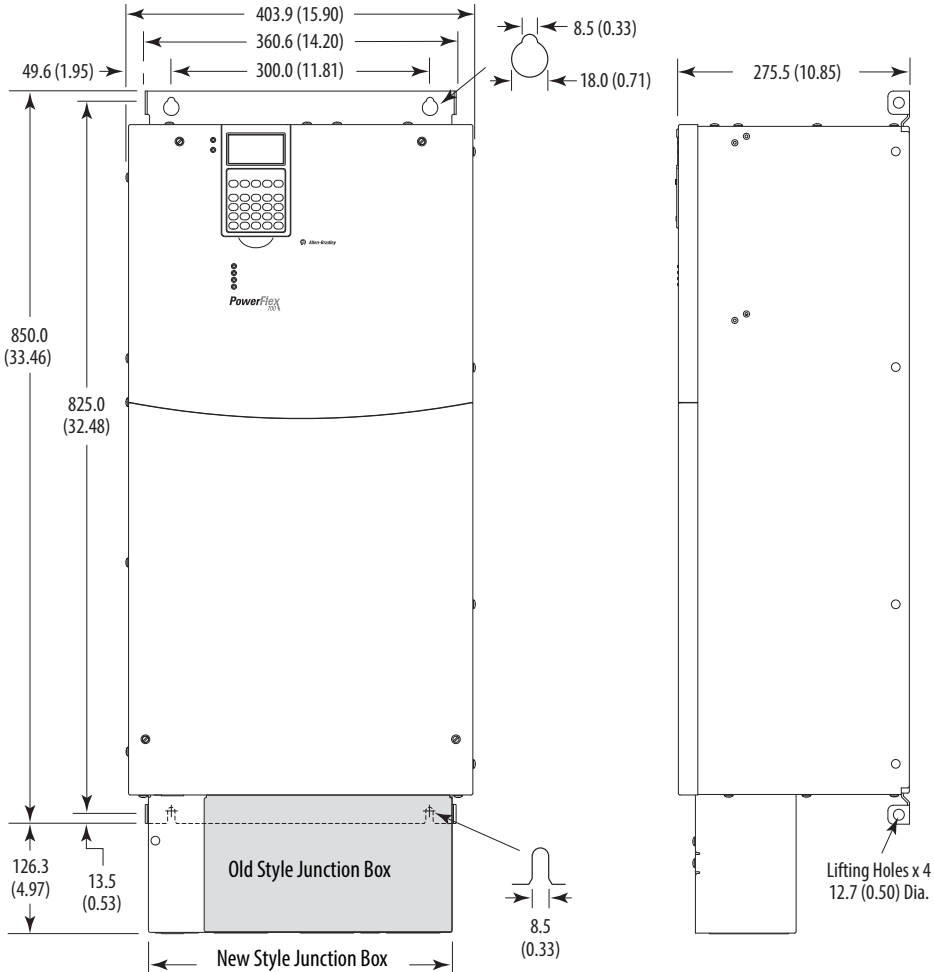
Junction Box can be removed if drive is mounted in a cabinet Dimensions are in millimeters and (inches)
