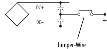
Common Mode Capacitor to Ground
